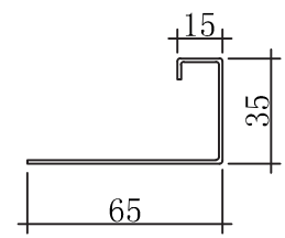
Optional Vanity Trim Door Surround
