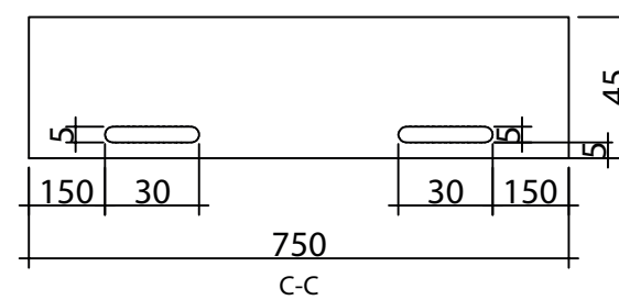
Fixing Tab
