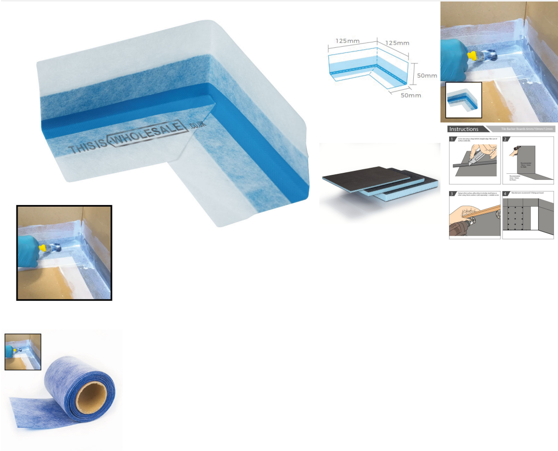
Tile Backer Board Waterproof Corner Joint - Membrane / Sealing Fleece Tanking Tape for Showers, Bathrooms, Wetrooms
